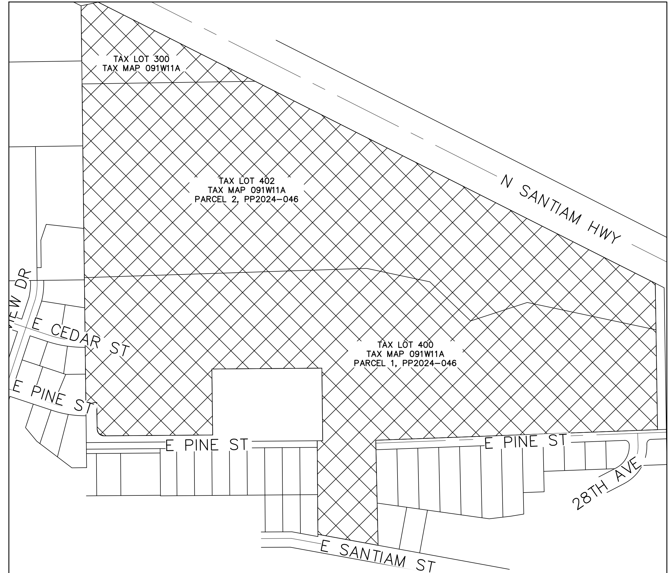
PROJECT LOCATION 1" = 250'
